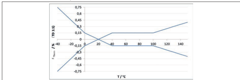
Fig. 32: Basic temperature error F_{TBasis} at TD 1 : 1
